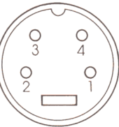
Figure D-7 Apple Desktop Bus pin-outs
