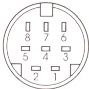
Figure D-3 Printer and modem port pin-outs
